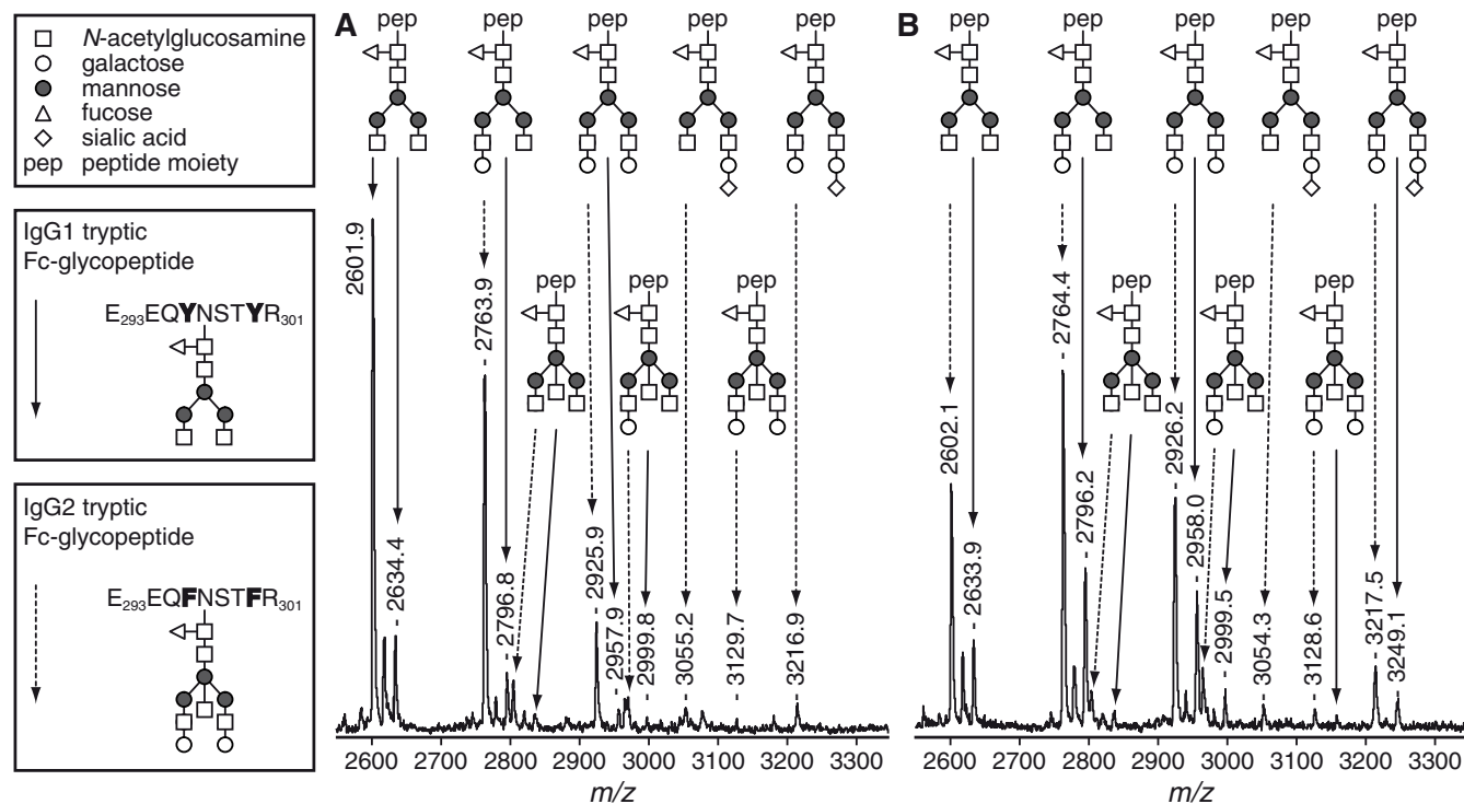
MALDI-TOF-MS analysis of tryptic glycopeptides of IgG1 and IgG2. A representative sample of an RA-patient before pregnancy (a) and in the third trimester (b) is shown. Glycopeptides derived from IgG1 and IgG2 were analyzed for galactosylation and sialylation in the reflection positive mode. Glycopeptides of IgG1 are indicated by continued arrows, while glycopeptides of IgG2 are indicated by striated arrows. Three glycoforms of IgG1 have been found to be below the detection limit of the MALDI-TOF-MS method in this sample as well as in several other samples.
